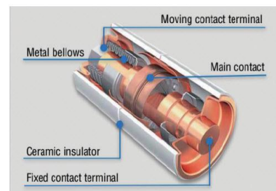
Vacuum Interrupter
